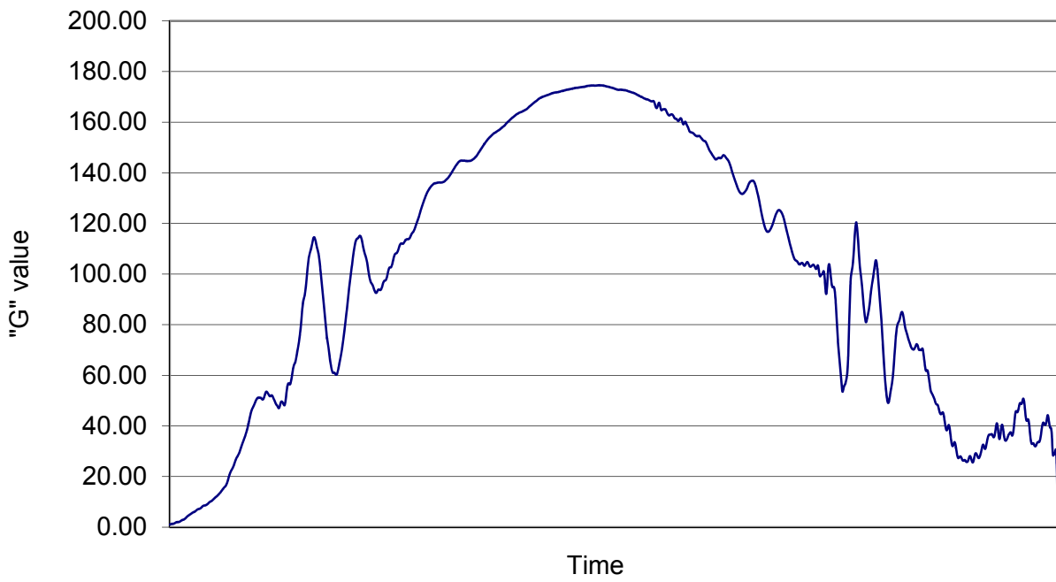
Deceleration Curve - Paver: Black 45mm
