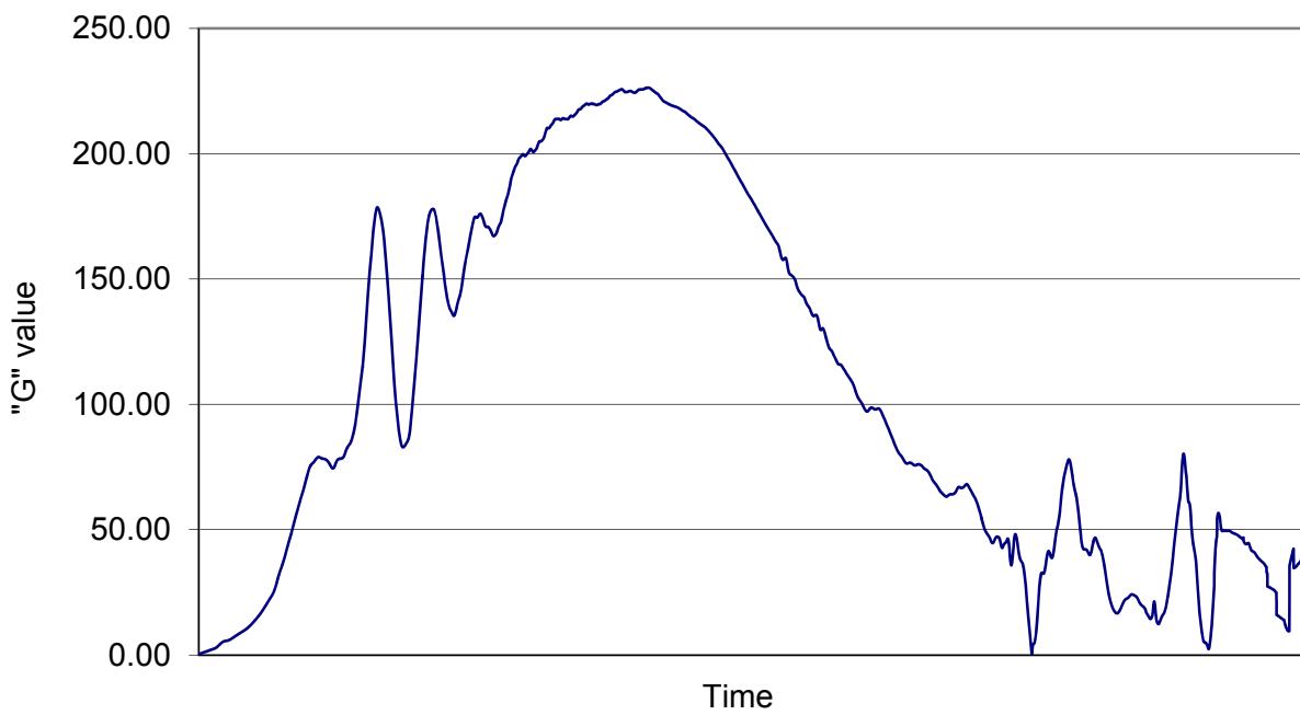
Deceleration Curve - Paver: Red 25mm
