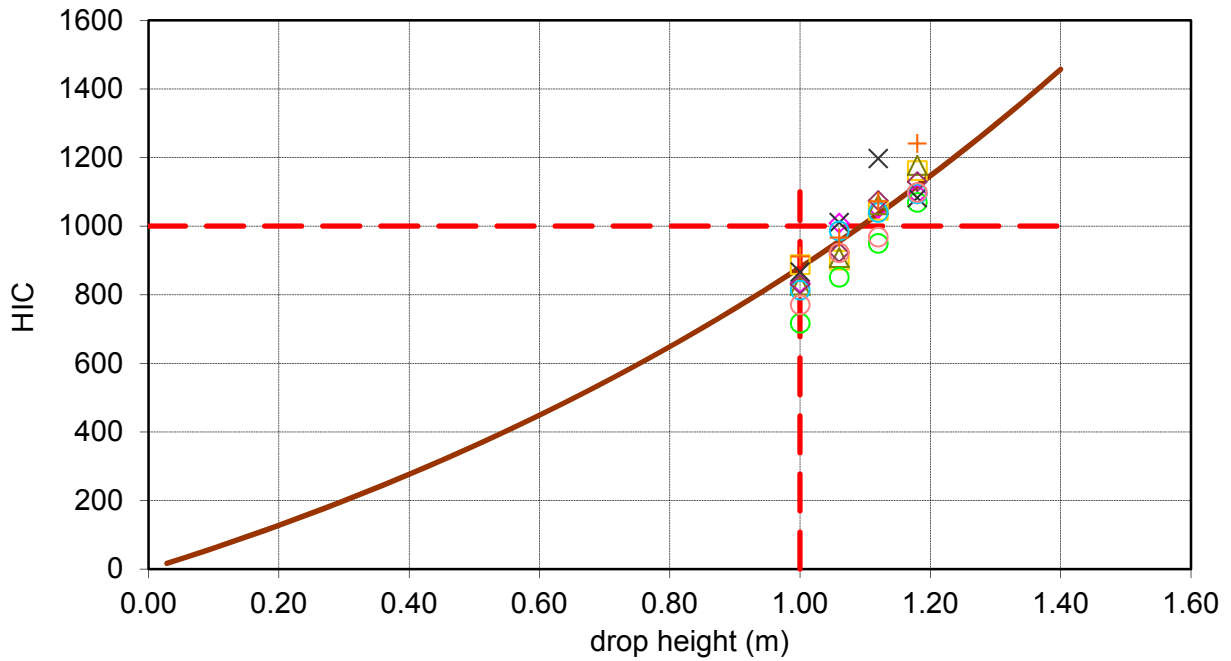
Head Injury Criterion Data - Tile: Red 37mm
