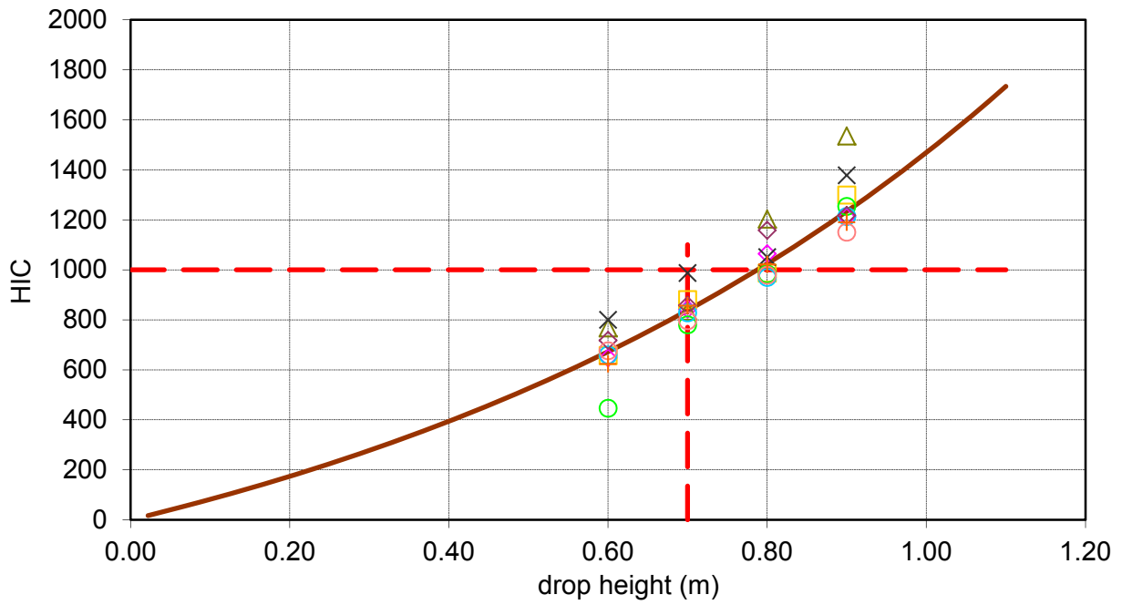
Head Injury Criterion Data - Tile: Black 25mm
