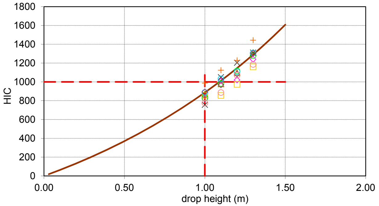
Head Injury Criterion Data - Paver: Black 45mm
