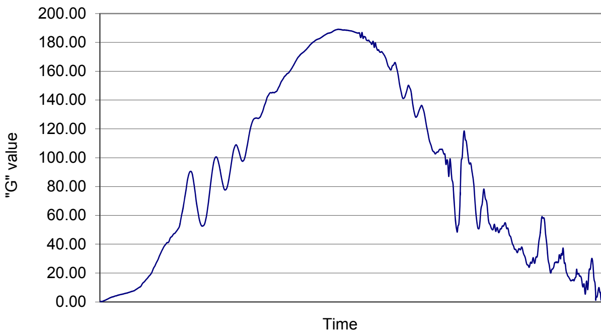
Deceleration Curve - Tile: Red 37mm
