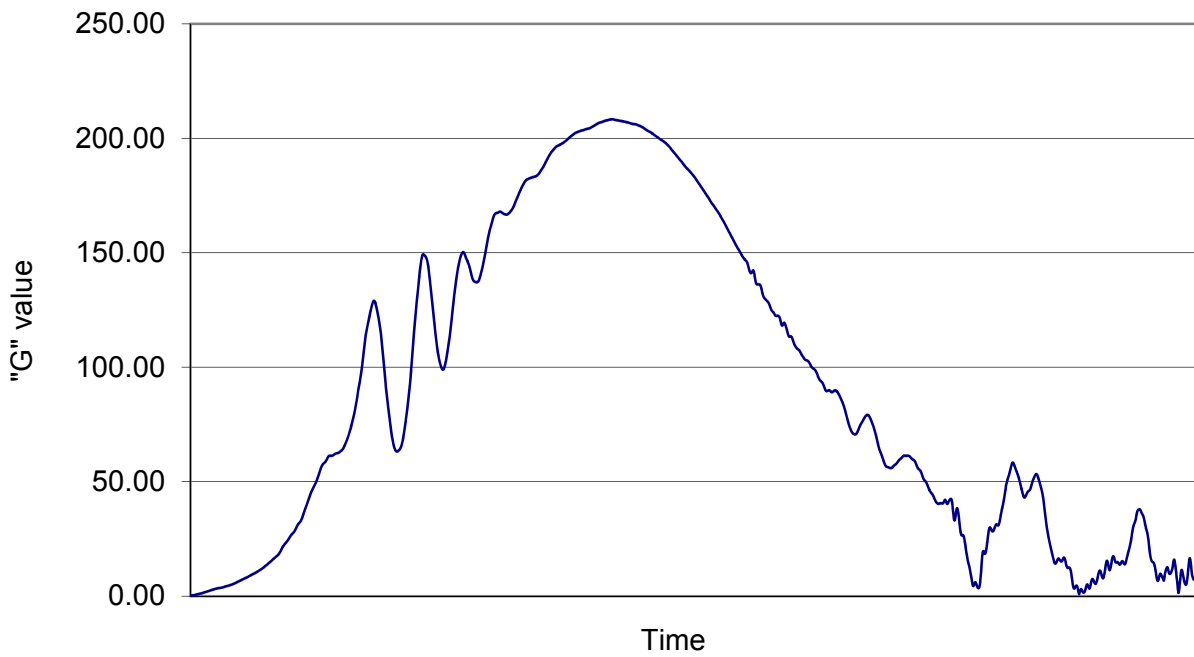
Deceleration Curve - Tile: Black25mm
