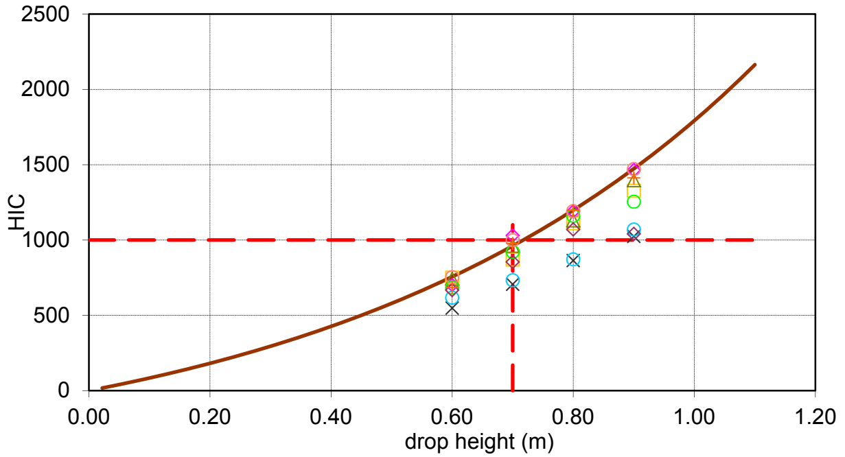
Head Injury Criterion Data - Paver: Red 25mm
